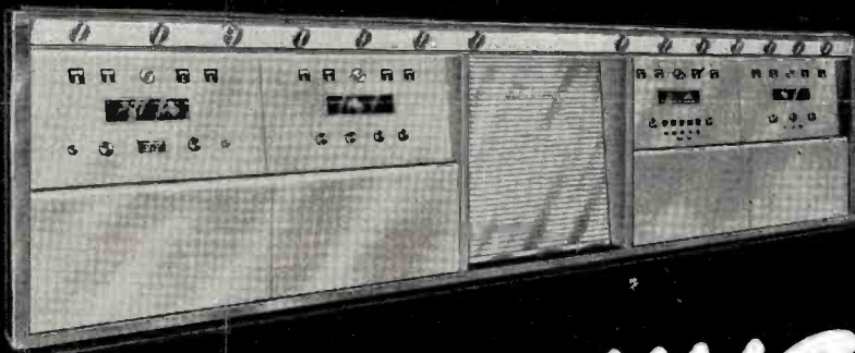
The New G-E 5-Kw Television Transmitter
